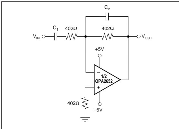
FIGURE 7. Inverting Bandpass Filter.
