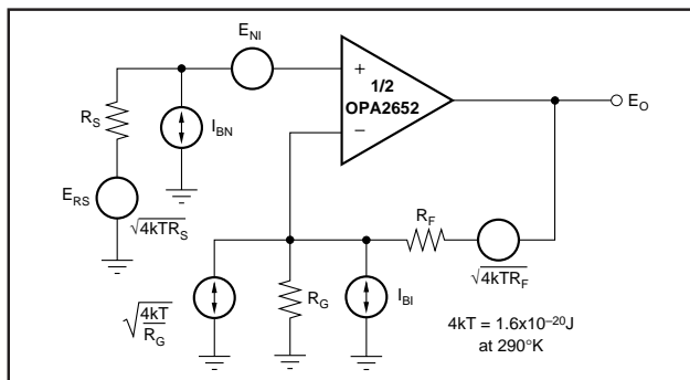
FIGURE 8. Op Amp Noise Analysis Model.
