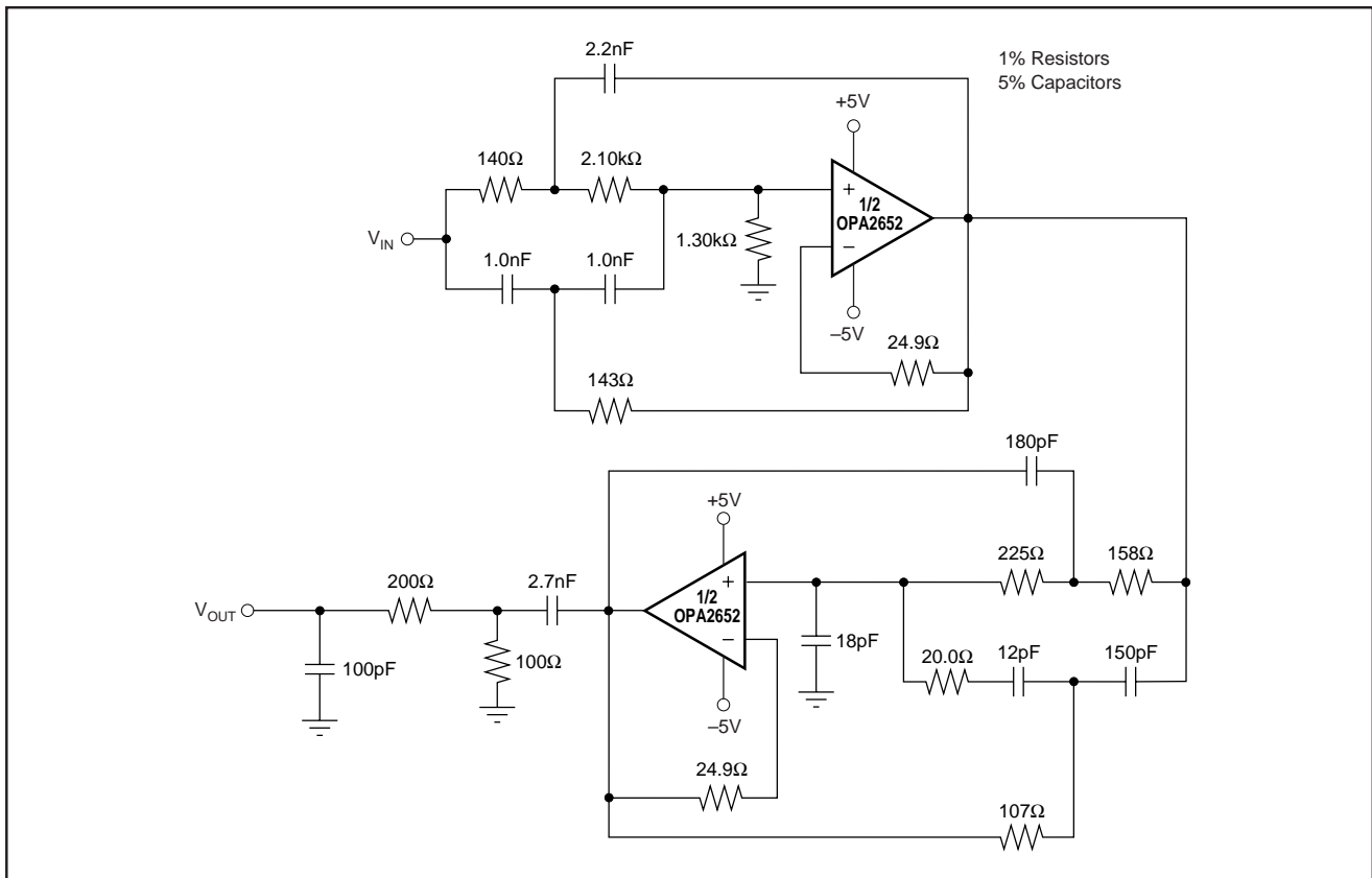
FIGURE 3. Bandpass Filter.
