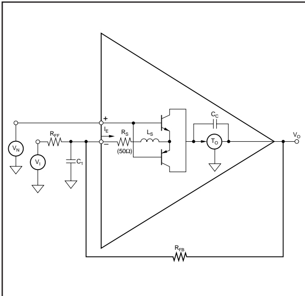
FIGURE 1. Equivalent Circuit.
