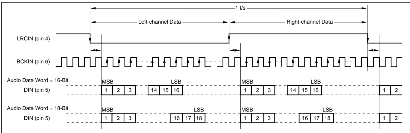
FIGURE 6. "I2S" Data Input Timing.
