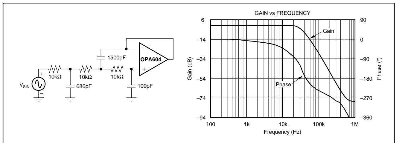
FIGURE 16. 3rd-Order LPF.
