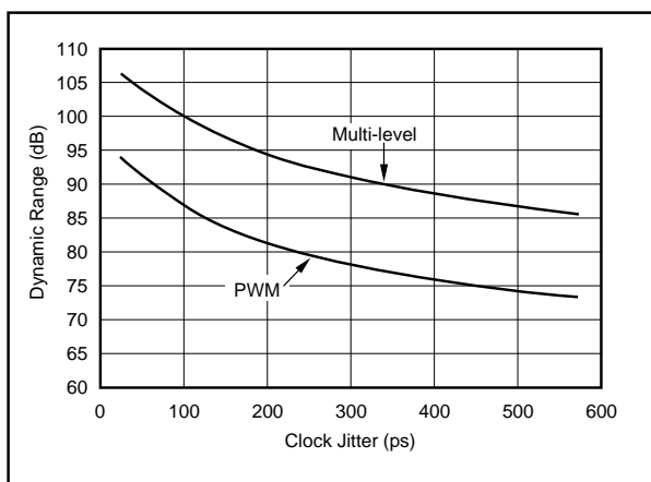
FIGURE 15. Simulation Results of Clock Jitter Sensitivity.
