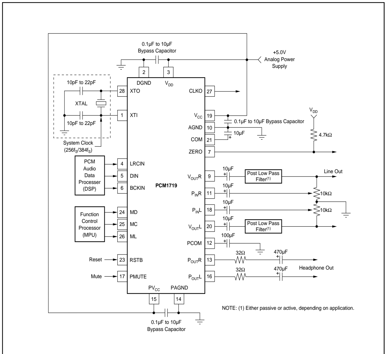
FIGURE 7. Typical Circuit Connection.
