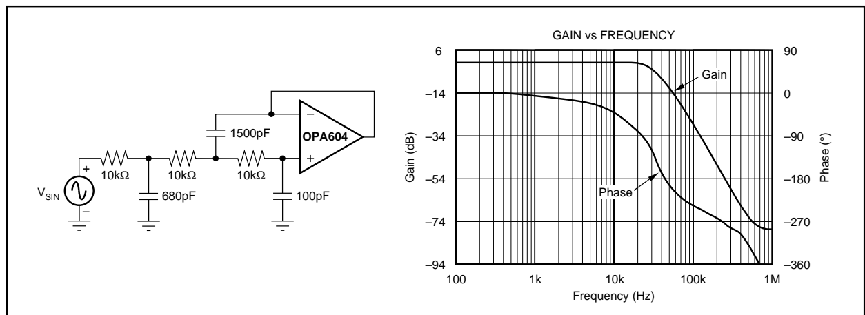
FIGURE 13. 3rd-Order LPF.
