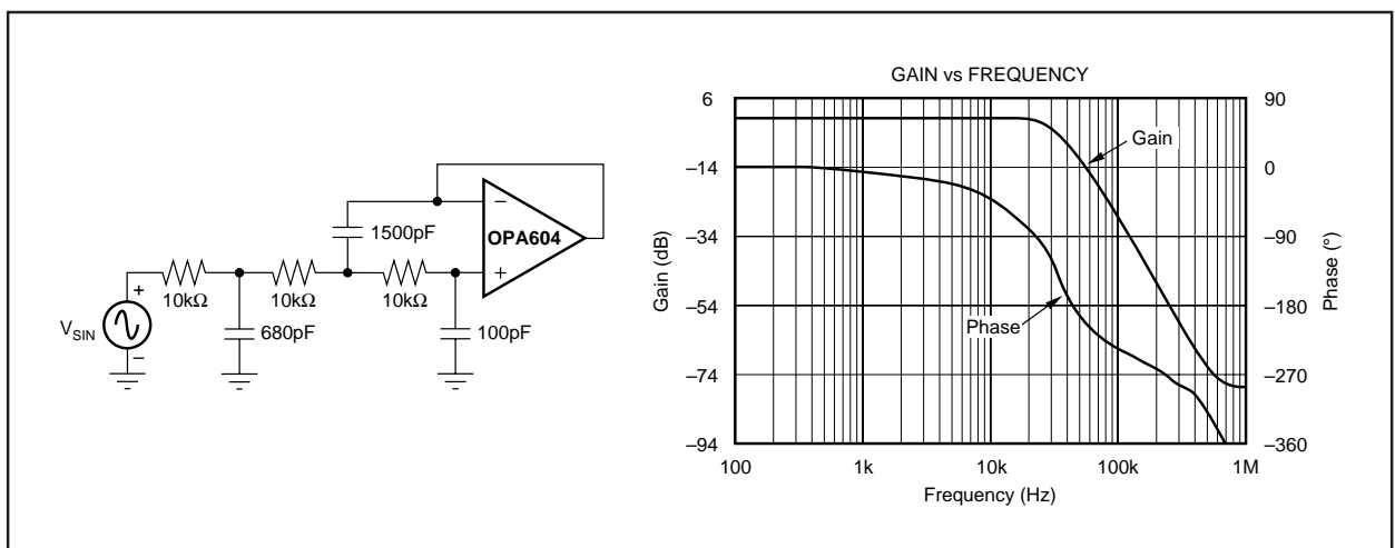
FIGURE 9. 3rd-Order LPF.
