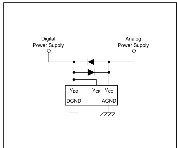
FIGURE 15. Latch-up Prevention Circuit.
