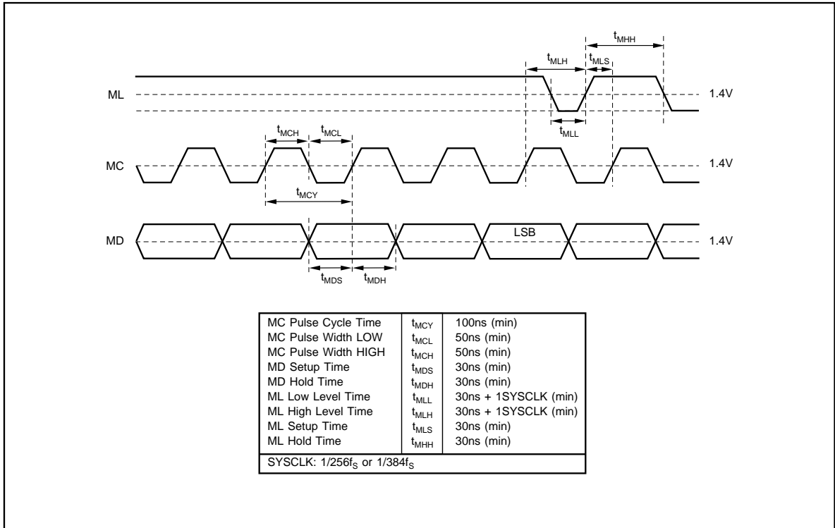
FIGURE 9. Program Register Input Timing.
