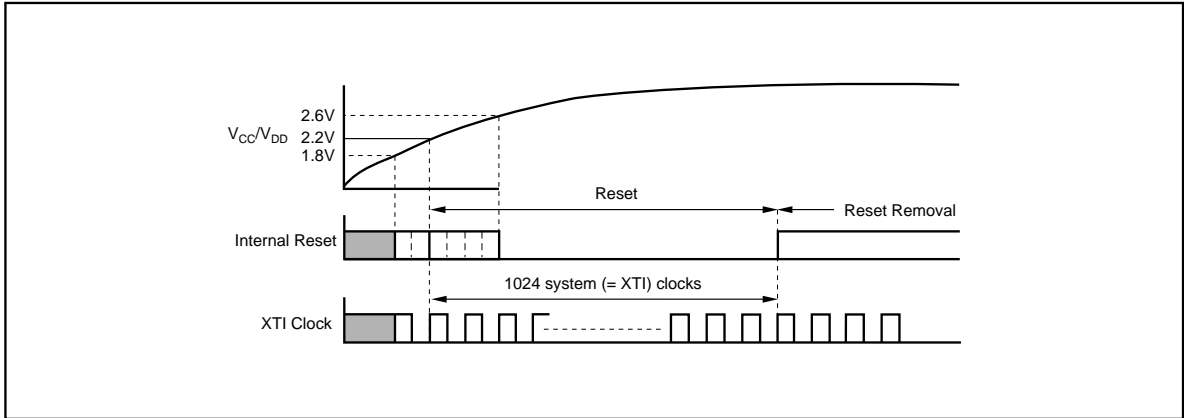
FIGURE 13. Internal Power-On Reset Timing.
