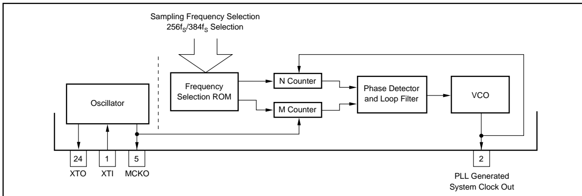
FIGURE 2. PLL Block Diagram.
