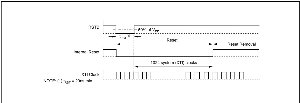
FIGURE 14. RSTB-Pin Reset Timing.
