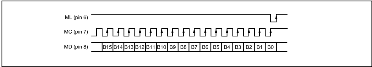
FIGURE 8. Three-Wire Serial Interface.
