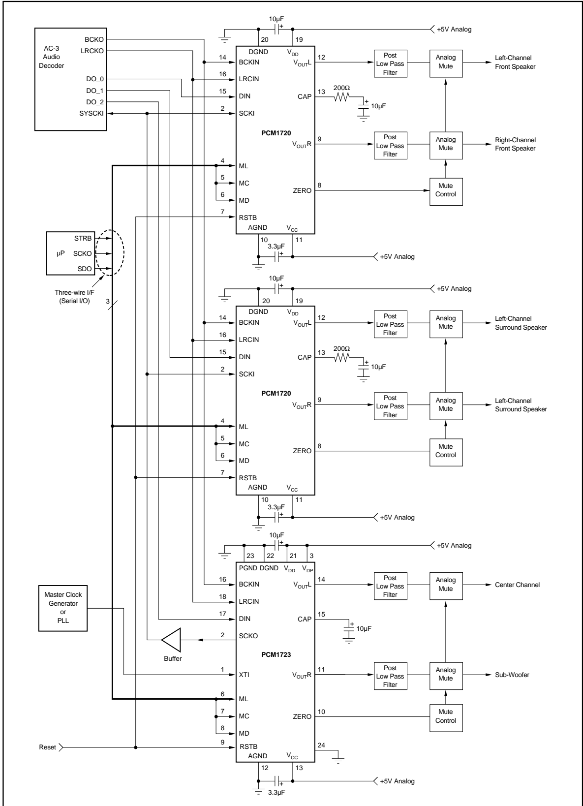
FIGURE 18. Connection Diagram for a 6-Channel AC-3 Application.
