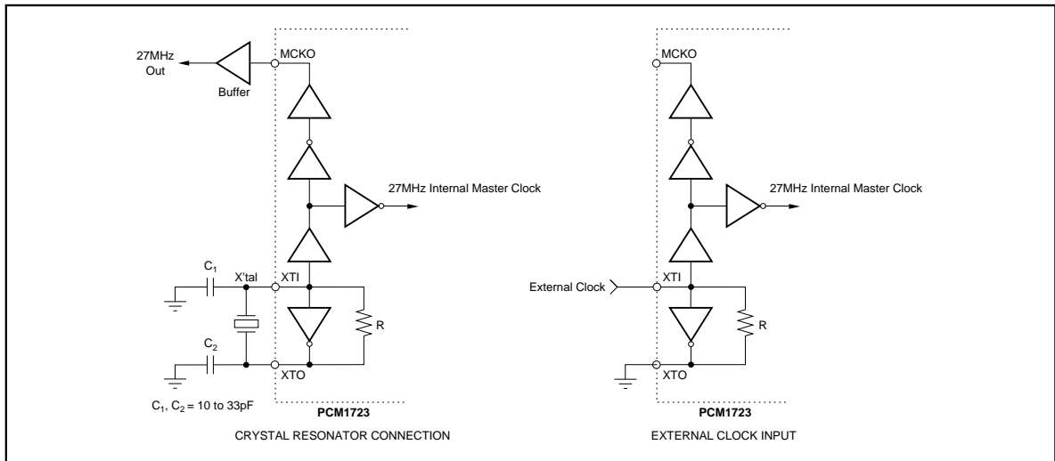
FIGURE 4. System Clock Connection.
