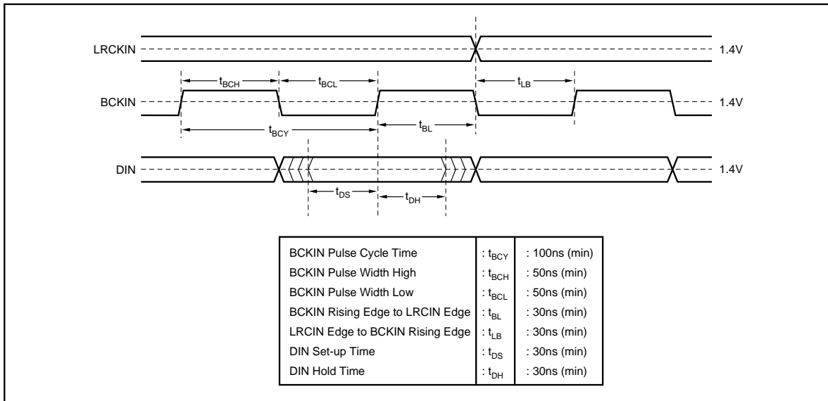
FIGURE 7. Audio Data Input Timing.
