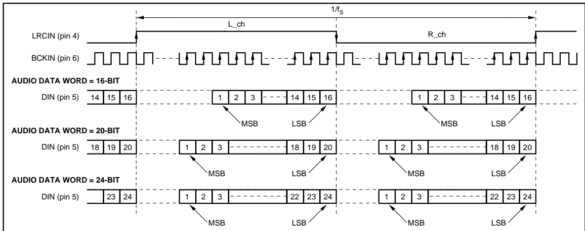
FIGURE 5. "Normal" Data Input Timing.
