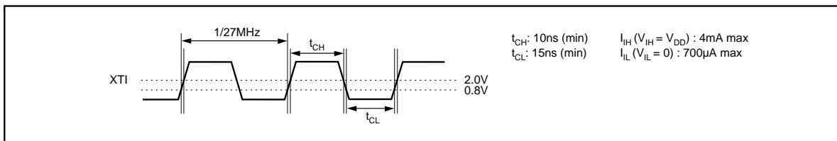
FIGURE 3. XTI Input Timing.
