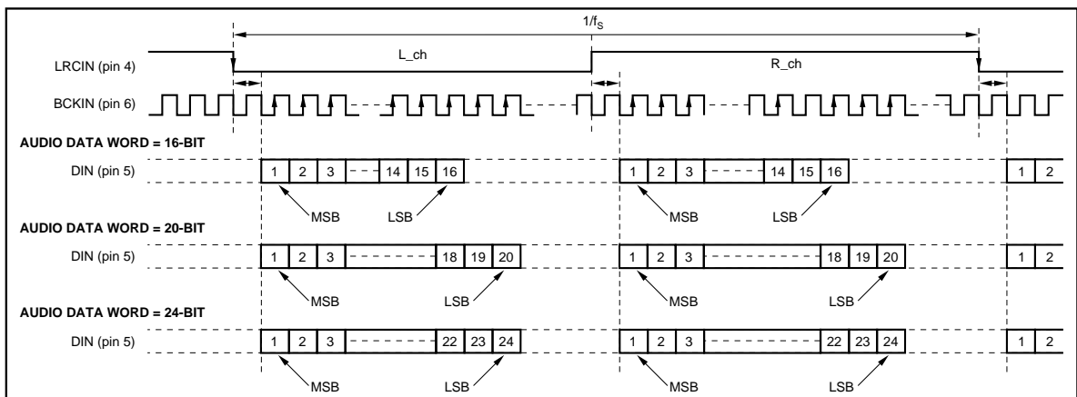
FIGURE 6. "I²S" Data Input Timing.
