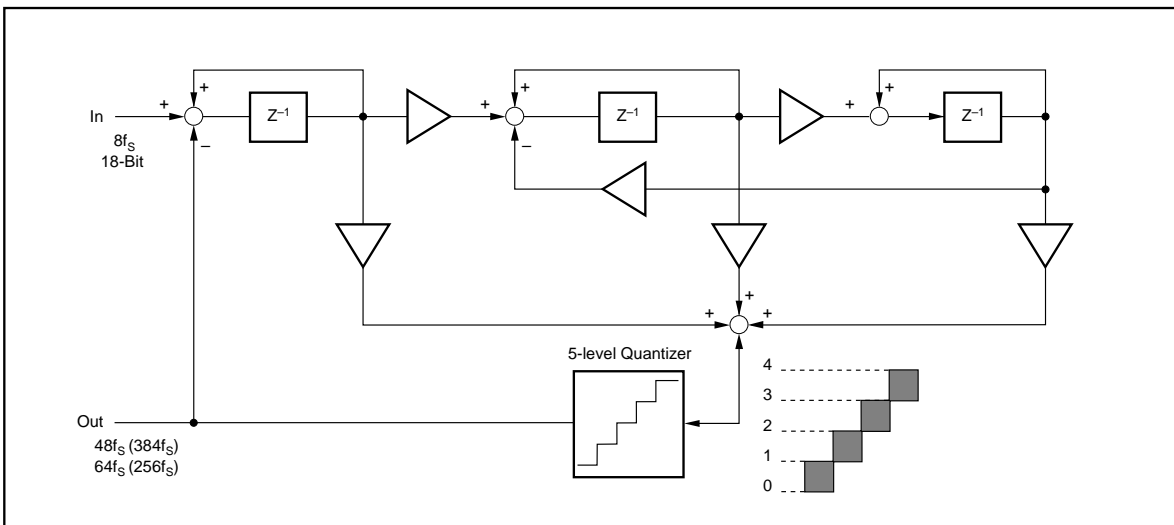
FIGURE 16. 5-Level \Delta\Sigma Modulator Block Diagram.
