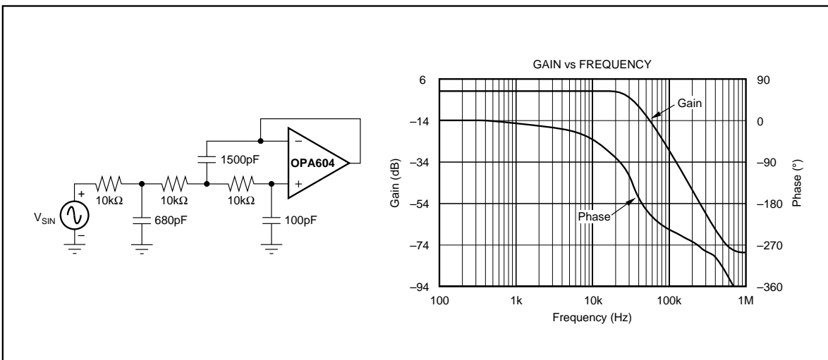
FIGURE 12. 3rd-Order LPF.
