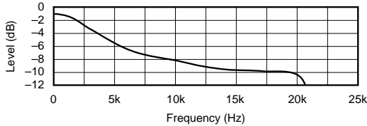
DE-EMPHASIS FREQUENCY RESPONSE (48kHz)
