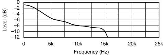
DE-EMPHASIS FREQUENCY RESPONSE (44.1kHz)
