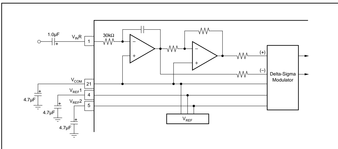
FIGURE 1. Analog Front-End (Single-Channel).
