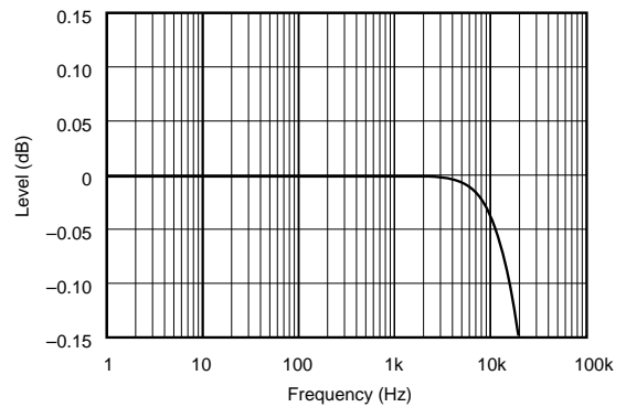
INTERNAL ANALOG FILTER FREQUENCY RESPONSE (1Hz-20kHz)
