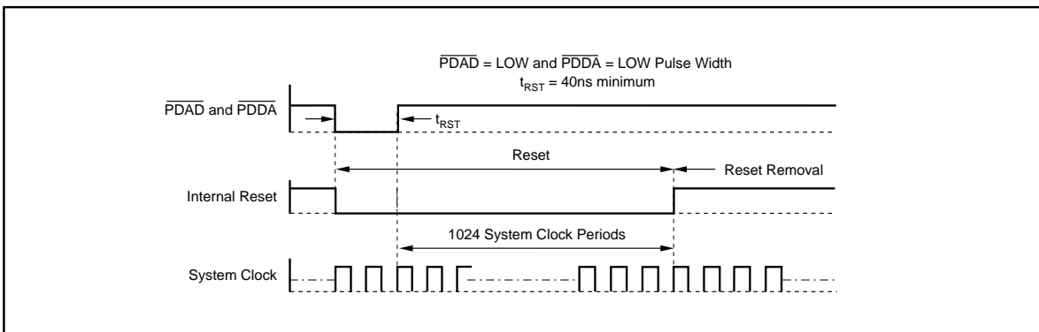
FIGURE 6. External Forced Reset Timing.
