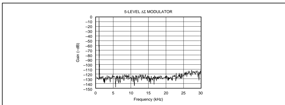
FIGURE 12. Quantization Noise Spectrum.
