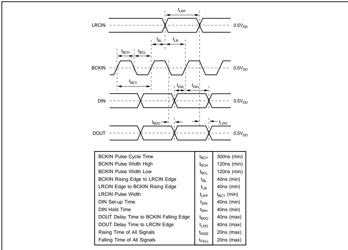
FIGURE 3. Audio Data Input/Output Timing.
