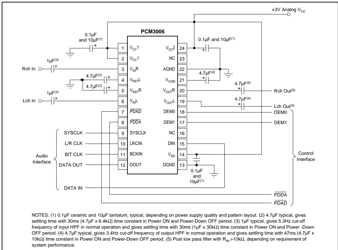
FIGURE 9. Typical Connection Diagram for PCM3006.
