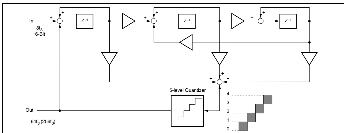
FIGURE 11. 5-Level \Delta\Sigma Modulator Block Diagram.
