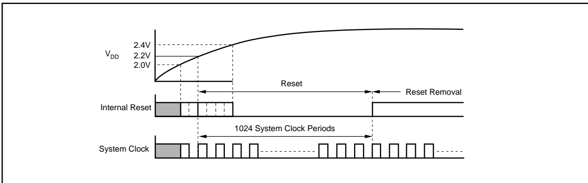
FIGURE 5. Internal Power-On Reset Timing.
