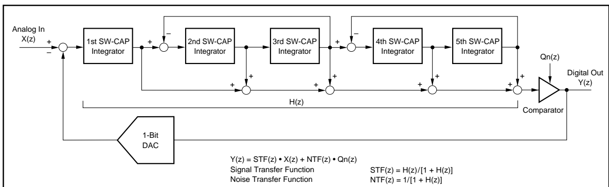
FIGURE 10. Simplified 5-Level Delta-Sigma Modulator.
