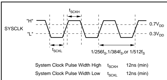
FIGURE 4. System Clock Timing.
