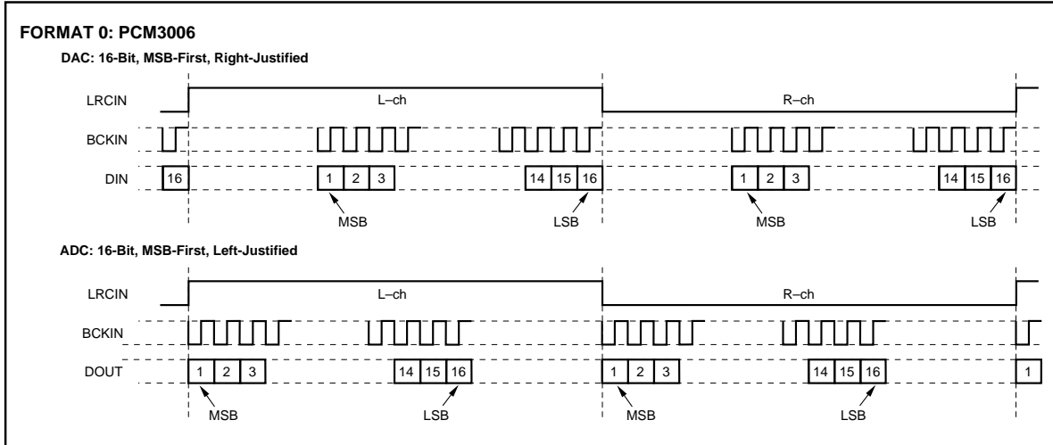
FIGURE 2. Audio Data Input/Output Format.
