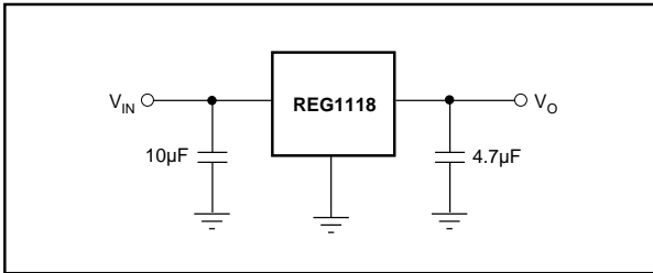
FIGURE 1. Basic Connections.
