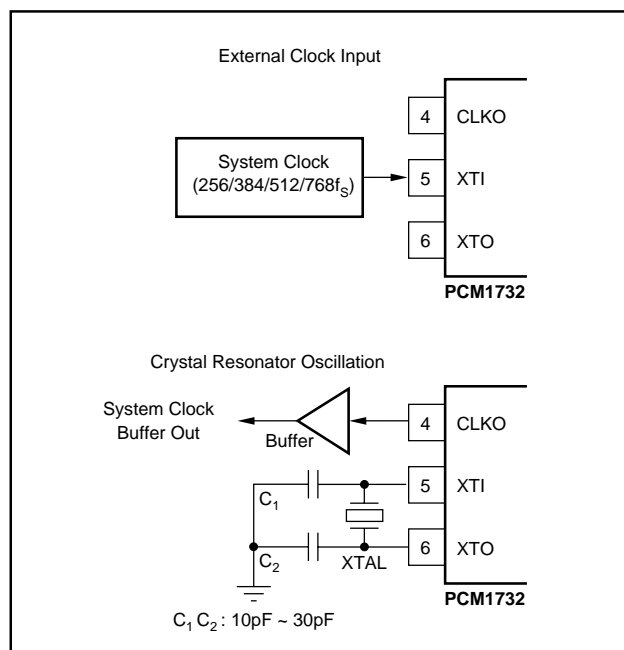
FIGURE 1. System Clock Connection.
