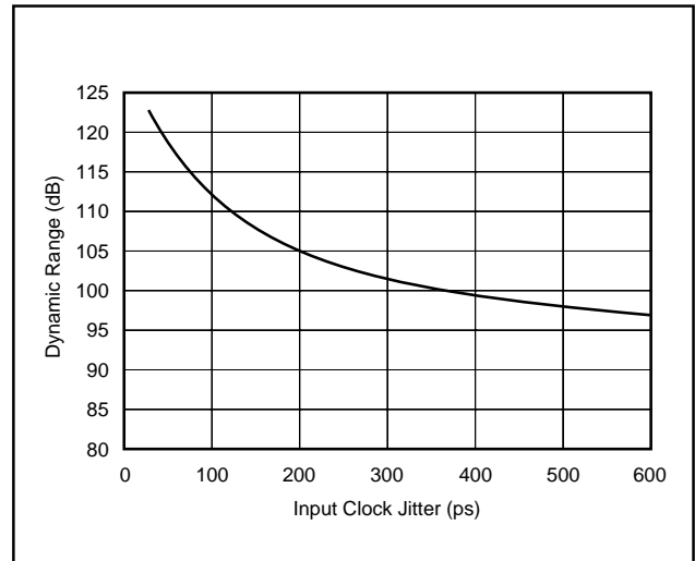
FIGURE 12. Jitter Sensitivity.
