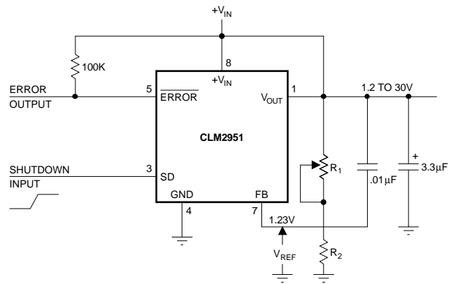
FIGURE 2. ADJUSTABLE REGULATOR
