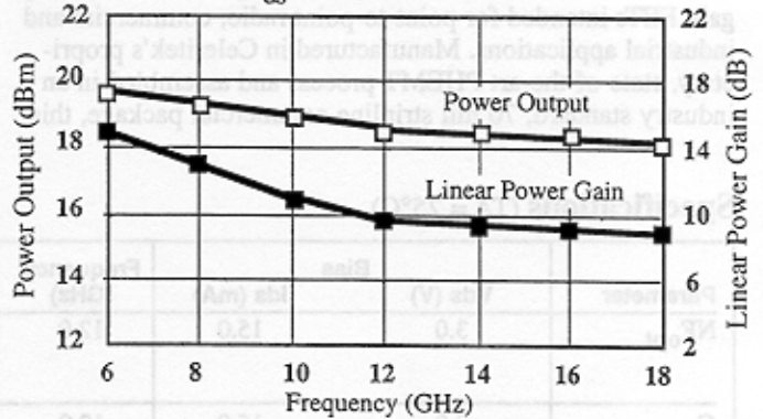
Power Output and Linear Power Gain vs Frequency V ds = 6V, I ds = 40 mA
