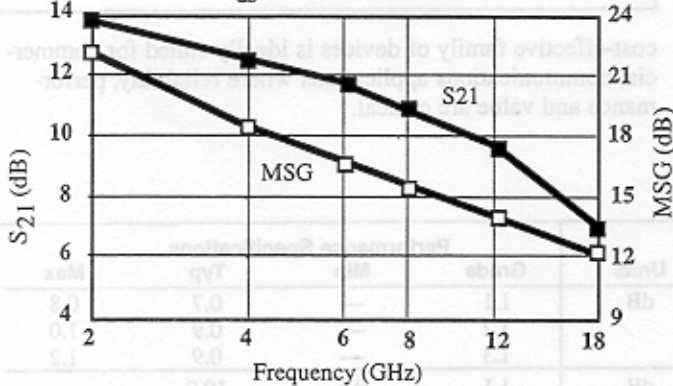
S 21 and MSG vs Frequency V ds = 3V, I ds = 15 mA
