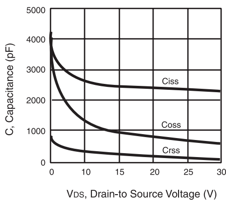
Figure 3. Capacitance
