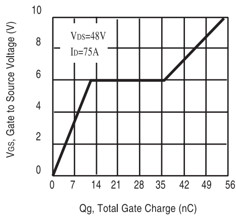
Figure 9. Gate Charge
