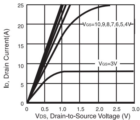
Figure 1. Output Characteristics
