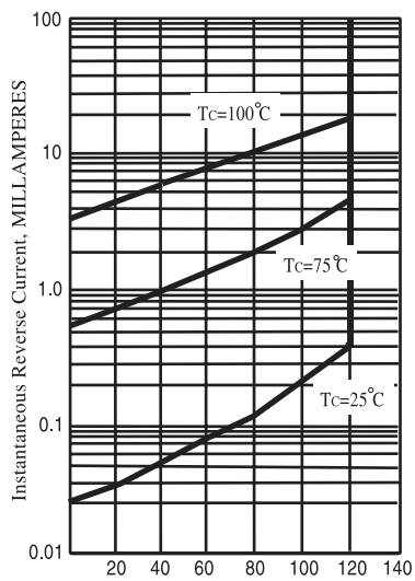
Percent of Rated Voltage Peak Reverse Voltage Figure 2. Typical Reverse Characteristics
