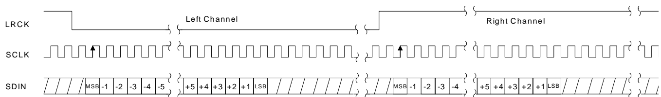
Figure 2. I²S Data
