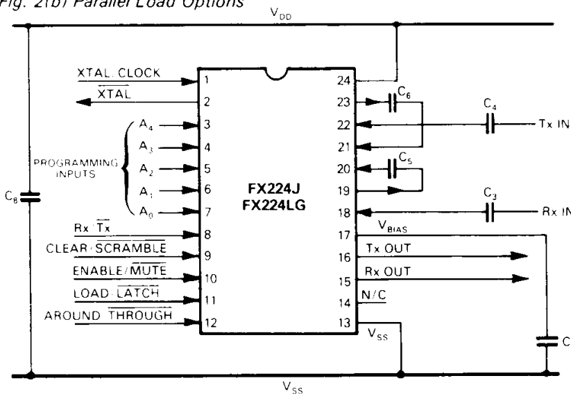
Fig. 2(b) Parallel Load Options
