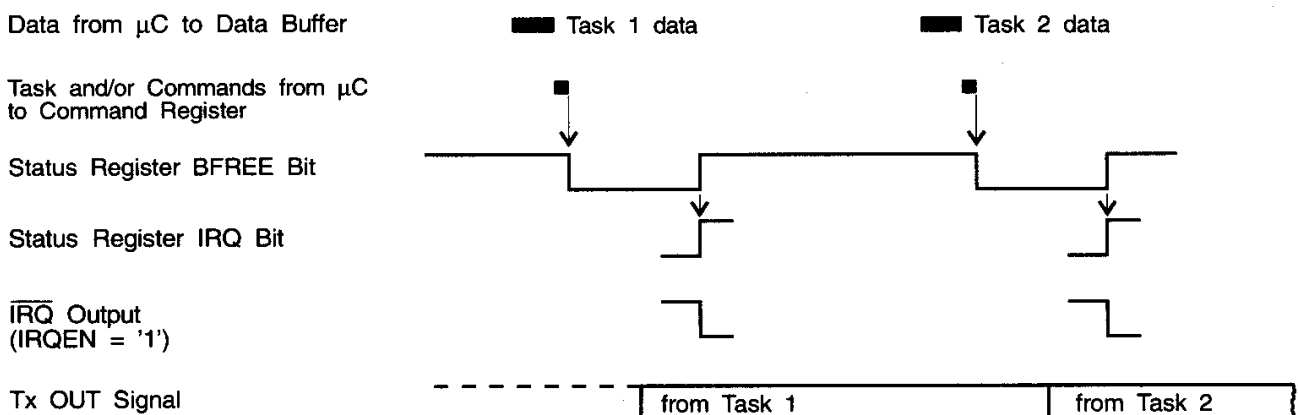
Fig.14 The Transmit Process
