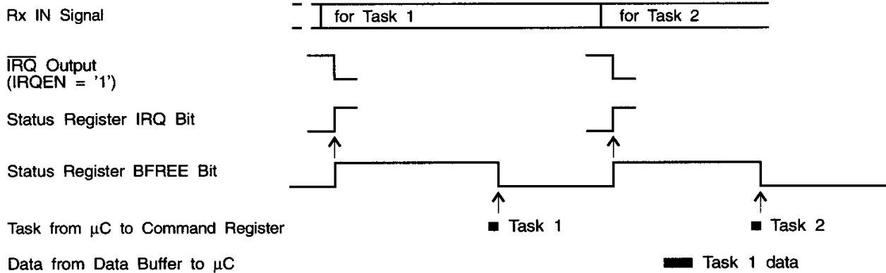
Fig.13 The Receive Process
