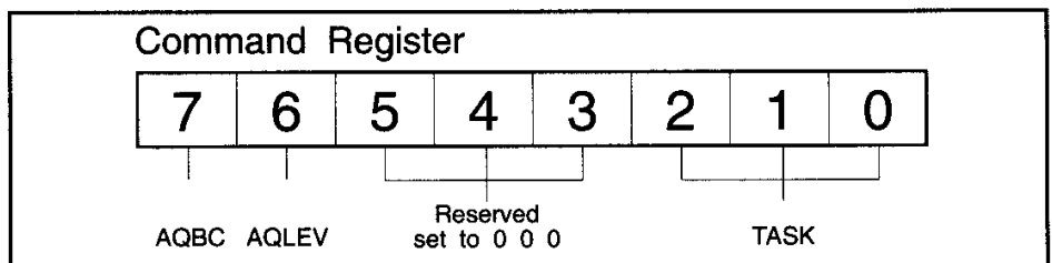
Fig. 12 The Command Register
