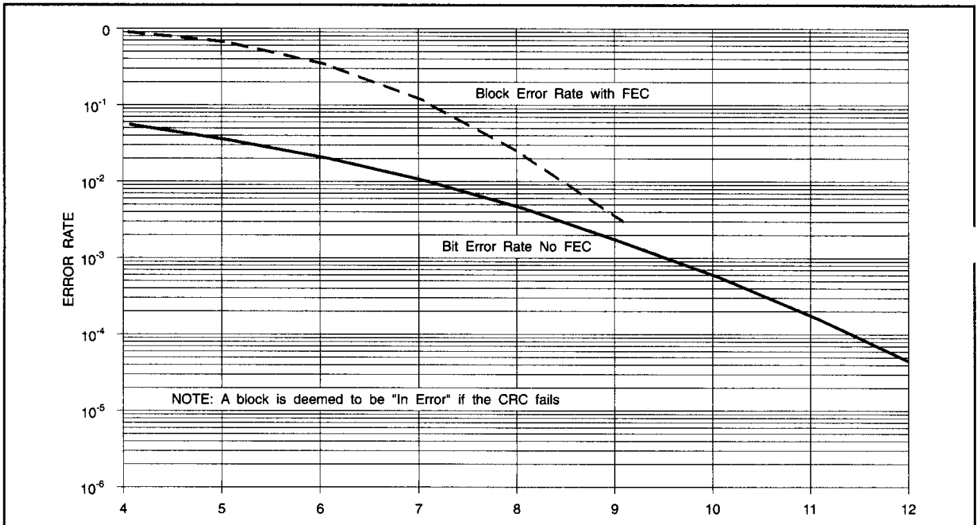
Fig.27 Typical Error Rates
