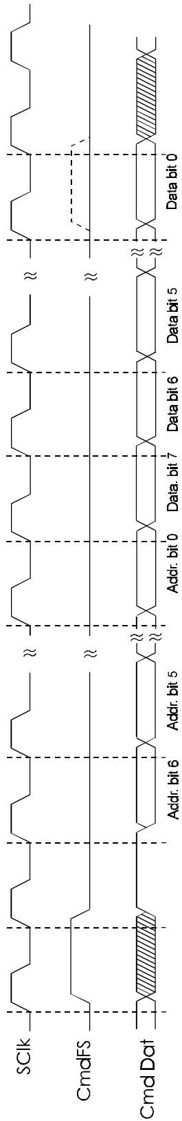
Figure 5b Command Write operation
