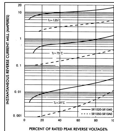
FIG.4-TYPICAL REVERSE CHARACTERISTICS
