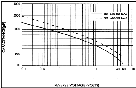
FIG.4-TYPICAL JUNCTION CAPACITANCE
