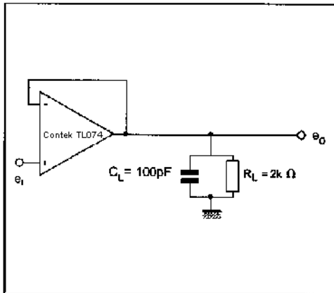
Figure 1 : Voltage Follower
