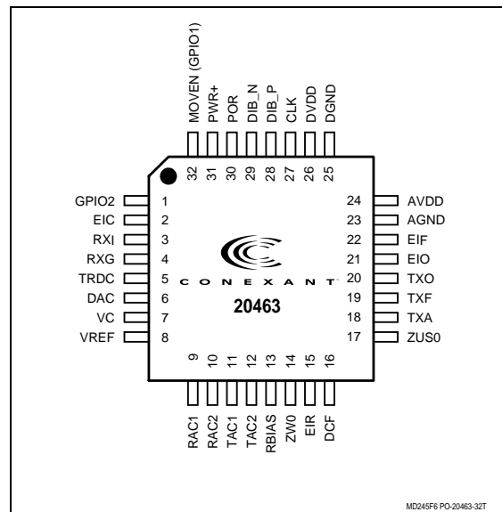
Figure 8. LSD (20463) 32-Pin TQFP Pin Signals
