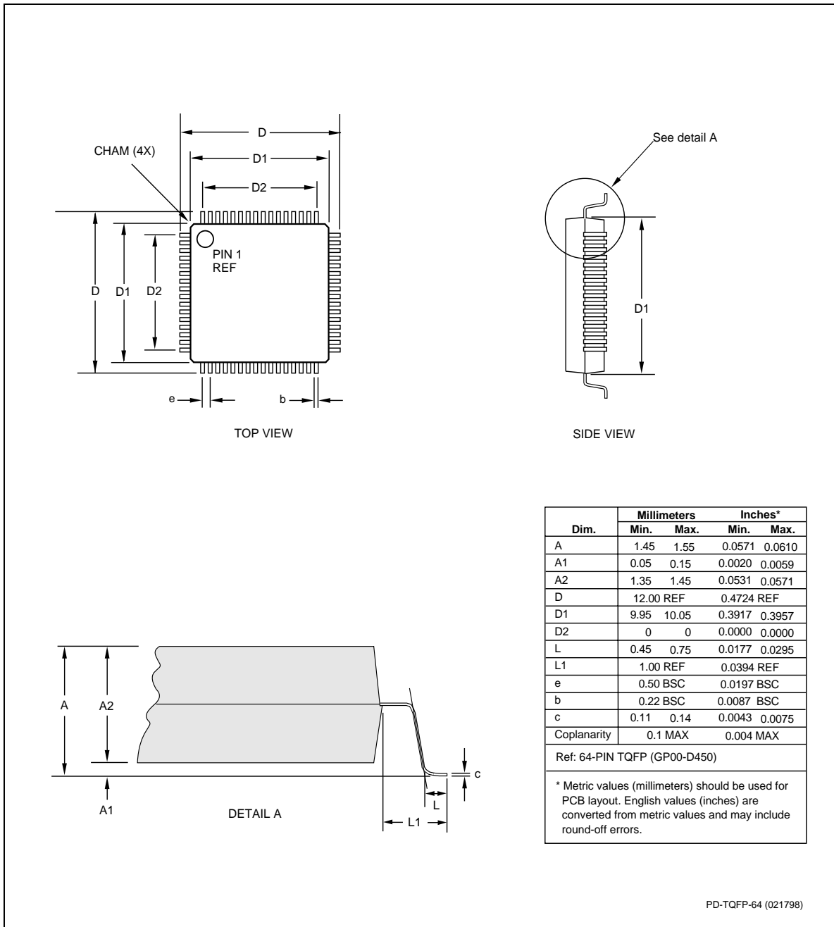
Figure 12. Package Dimensions - 64-Pin TQFP
