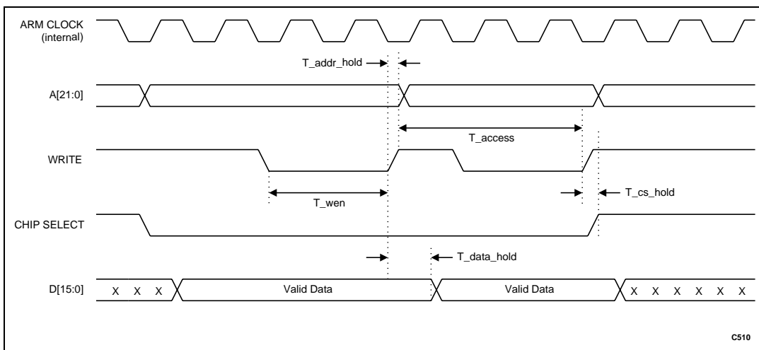
Figure 4. EXB Write Timing Diagram
