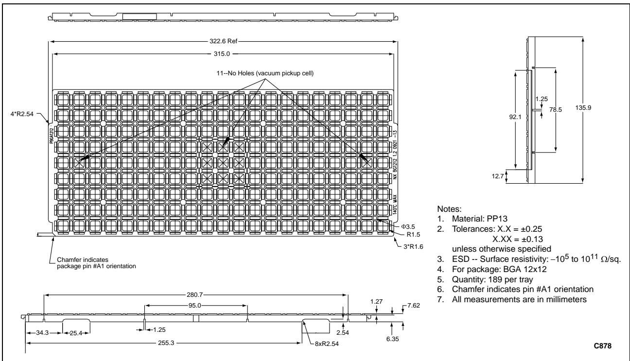
Figure 22. BP 160-Pin μBGA Shipping Tray Dimensions
