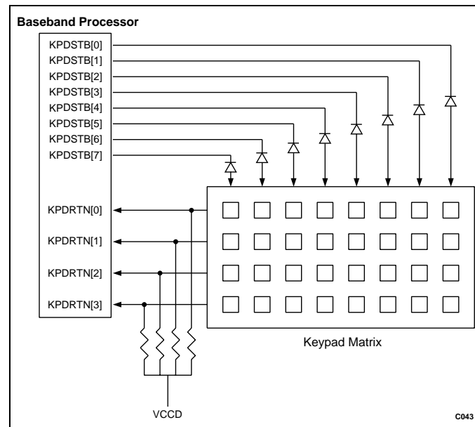
Figure 7. Typical Keypad Interface Circuit
