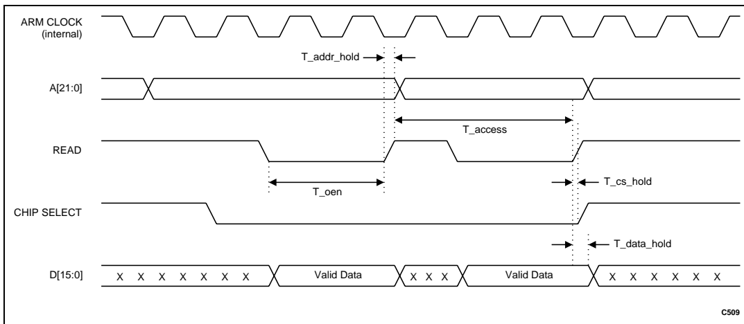
Figure 3. EXB Read Timing Diagram
