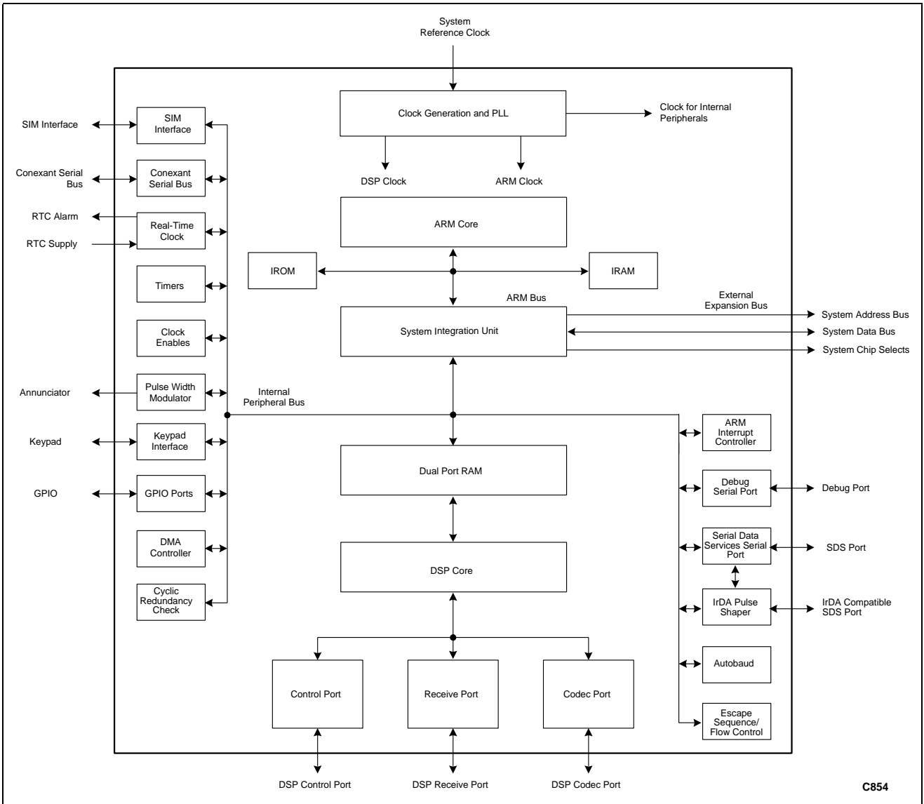
Figure 1. BP Block Diagram
