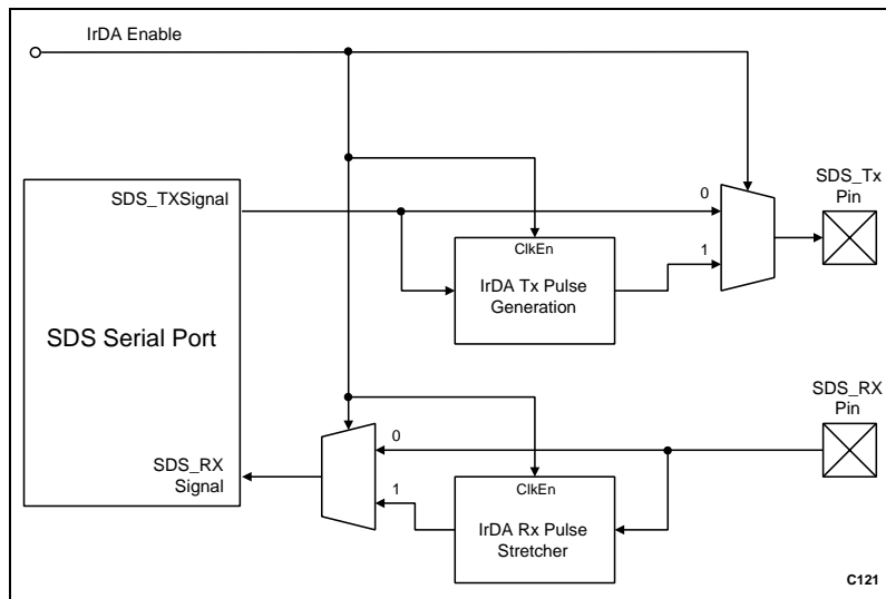
Figure 6. IrDa Pulse Shaper Functional Block Diagram
