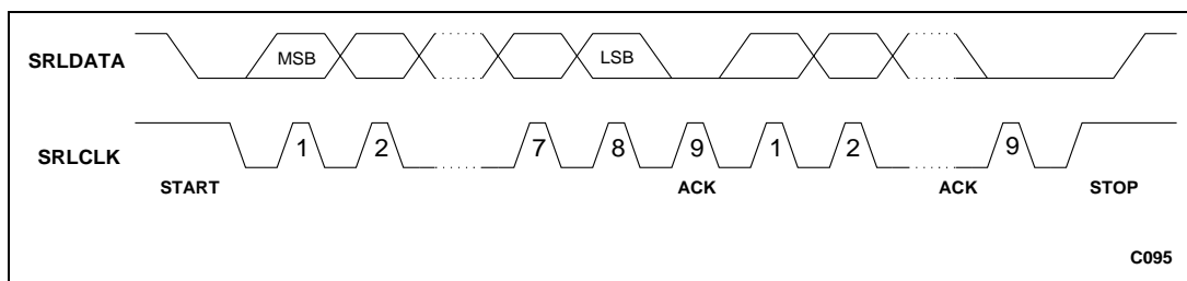
Figure 12. Serial Interface Data Format Diagram
