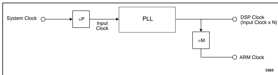
Figure 5. PLL Functional Block Diagram
