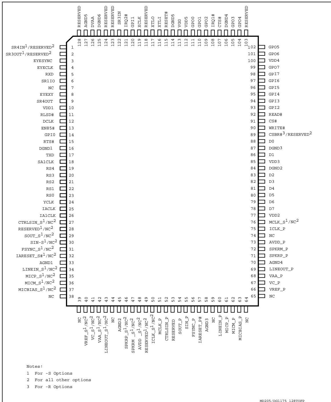
Figure 4. Pin Signals - 128-Pin TQFP
