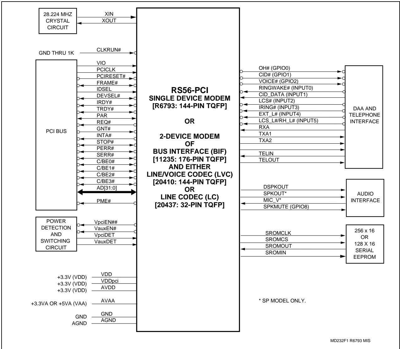
Figure 2. RS56-PCI Major Interface Signals
