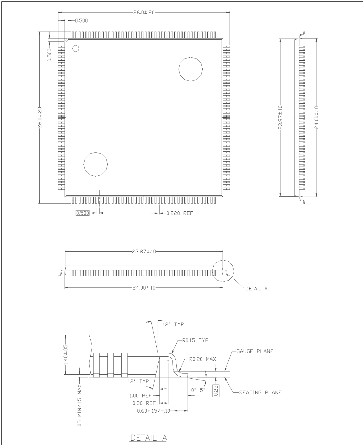
Figure 11. Package Dimensions - 176-Pin TQFP
