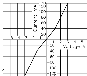
Voltage vs. current characteristics of output at MOS FET portion Measured portion: across terminals 5,7 and 6,8 pin Ambient temperature: 25°C
