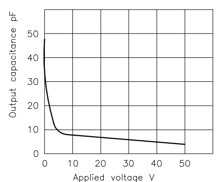
Applied voltage vs. output capacitance Across terminals 5,7 and 6,8 pin Frequency: 1MHz; Ambient temperature: 25°C
