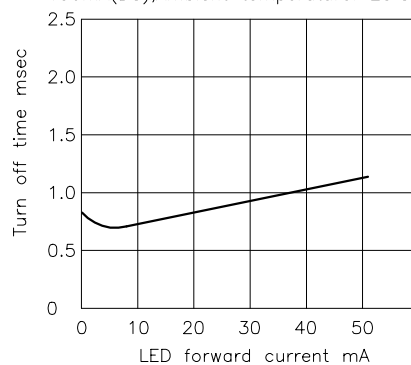
LED forward current vs. turn off time Across terminals 3 and 4 pin; Load voltage: 400V(DC); Continuous load current: 130mA(DC); Ambient temperature: 25°C
