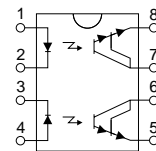
LDA211 Pinout
