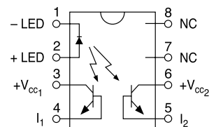
LOC112 Pinout
