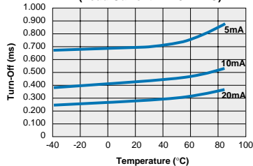
TS118 Typical Turn-Off vs. Temperature (Load Current = 120mADC)
