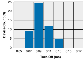
TS190 Typical Turn-Off Time (N=50 Ambient Temperature = 25°C) (Load Current = 150mADC; I F = 5mADC)
