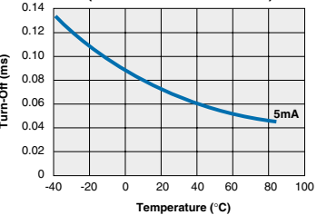
TS190 Typical Turn-Off vs. Temperature (Load Current = 150mADC)
