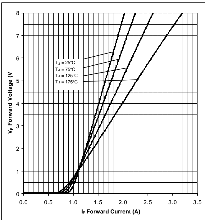
Figure 1. Forward Characteristics
