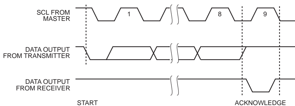
Figure 4. Acknowledge Timing
