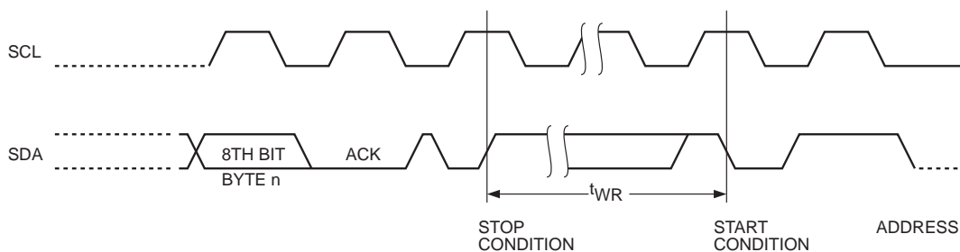
Figure 3. Start/Stop Timing
