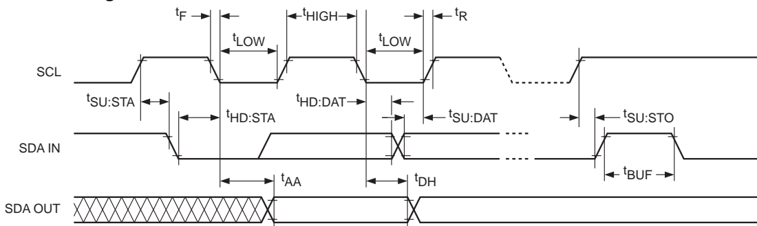
Figure 1. Bus Timing
