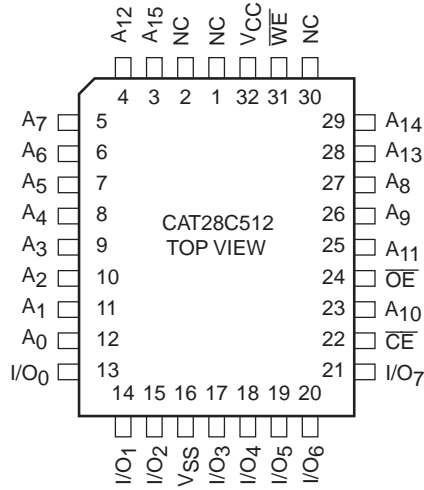
PLCC Package (N)
