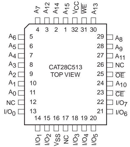
PLCC Package (N)
