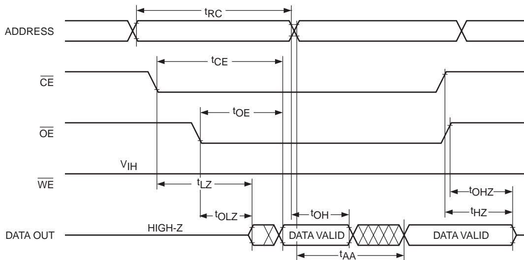
Figure 3. Read Cycle
