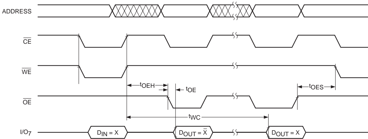
Figure 7. \overline{\text{DATA}} Polling
