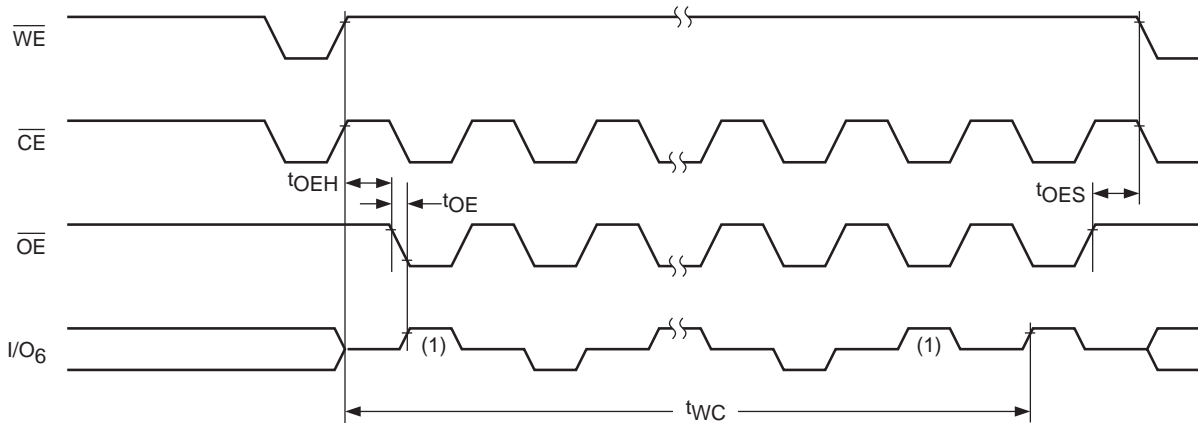
Figure 8. Toggle Bit
