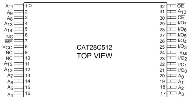
TSOP Package (8mmx20mm) (T)
