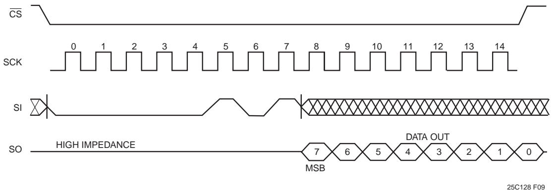
Figure 5. RDSR Timing
