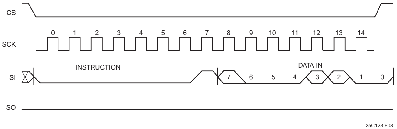
Figure 7. WRSR Timing
