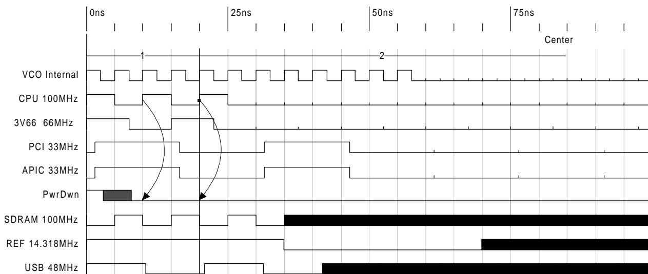
Figure 4. W147G PWRDWN# Timing Diagram [8, 9, 10, 11]
