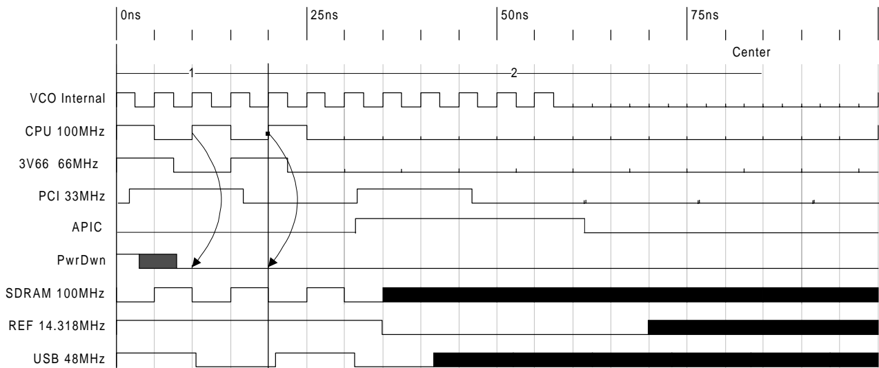
Figure 4. PWRDWN# Timing Diagram [2, 3, 4, 5]
