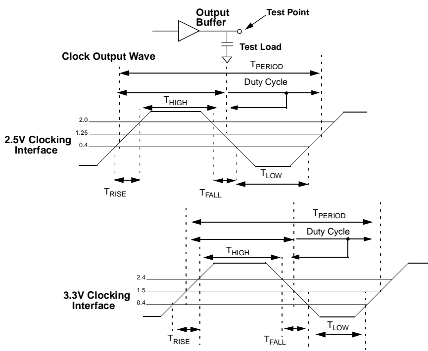
Figure 8. Output Buffer
