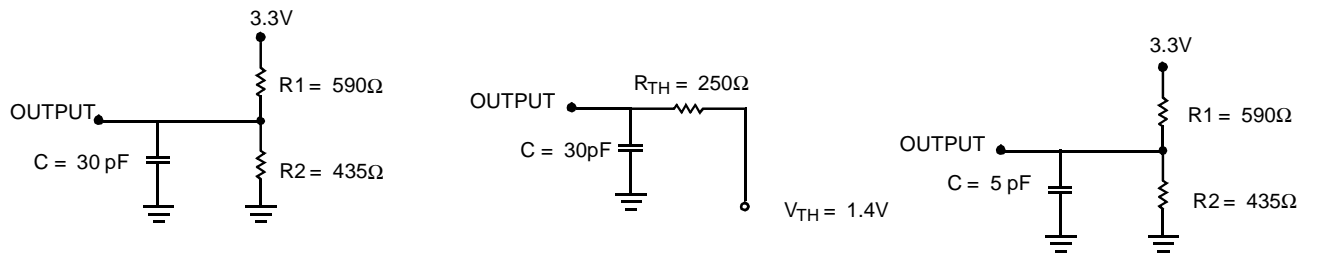
(a) Normal Load (Load 1) (b) Thévenin Equivalent (Load 1) (c) Three-State Delay (Load 2) (Used for t LZ , t HZ , t HZWE , & t LZWE including scope and jig)
