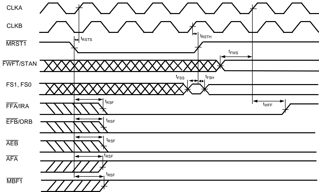
FIFO1 Reset Loading X1 and Y1 with a Preset Value of Eight [12]
