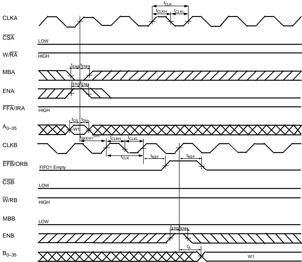
\overline{\text{EFB}} Flag Timing and First Data Read Fall Through when FIFO1 is Empty (CY Standard Mode) [20]
