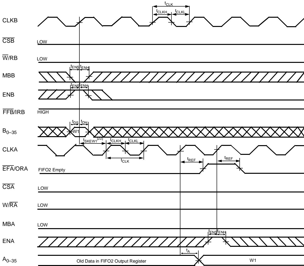
ORA Flag Timing and First Data Word Fall Through when FIFO2 is Empty (FWFT Mode) [21]
