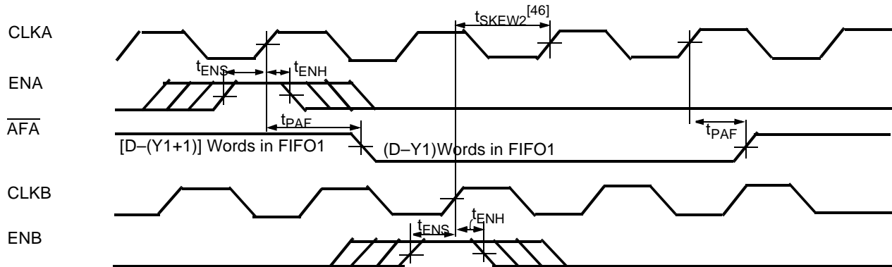
Timing for \overline{\text{AFA}} when FIFO1 is Almost Full (CY Standard and FWFT Modes) [38, 42, 44, 45]
