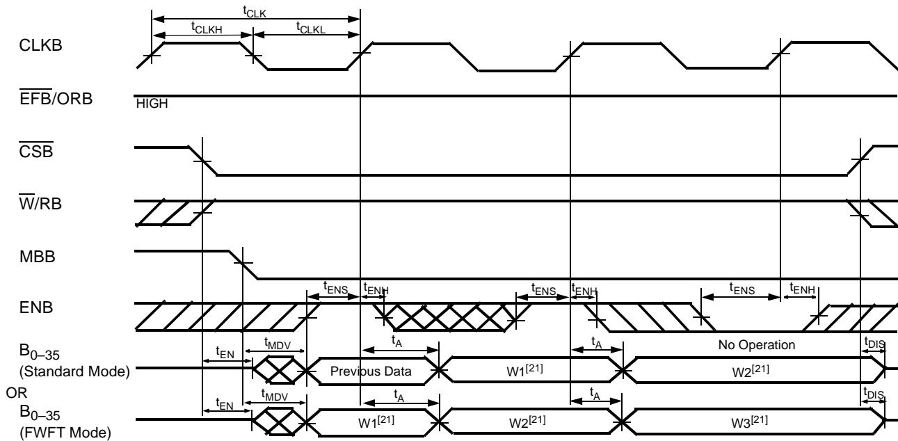
Port B Long-Word Read Cycle Timing for FIFO1 (CY Standard and FWFT Modes) [22]
