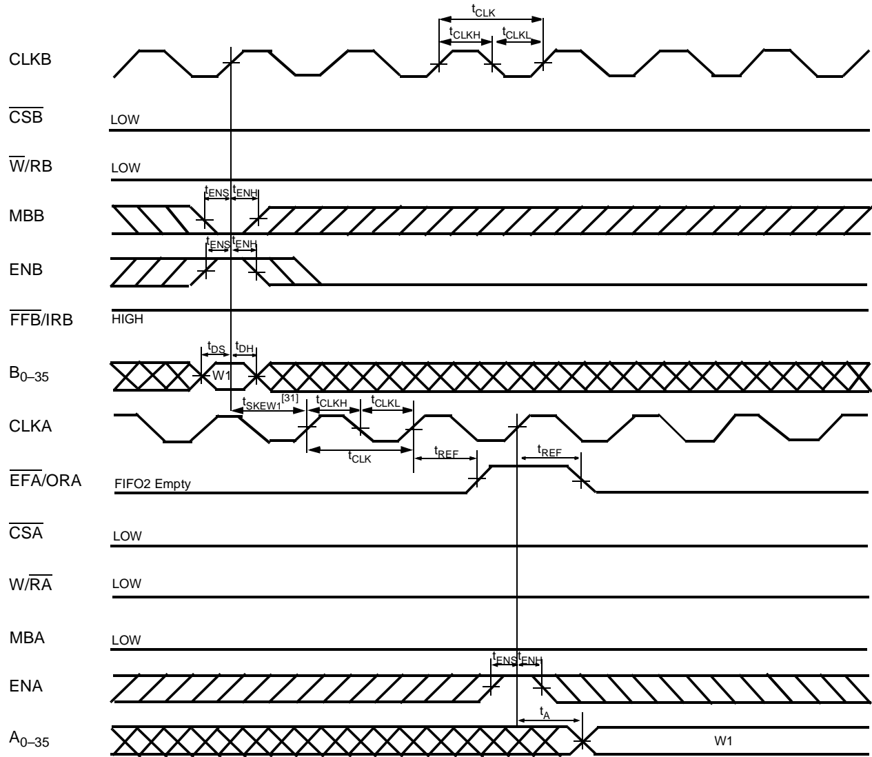
EFA Flag Timing and First Data Read when FIFO2 is Empty (CY Standard Mode) [29]
