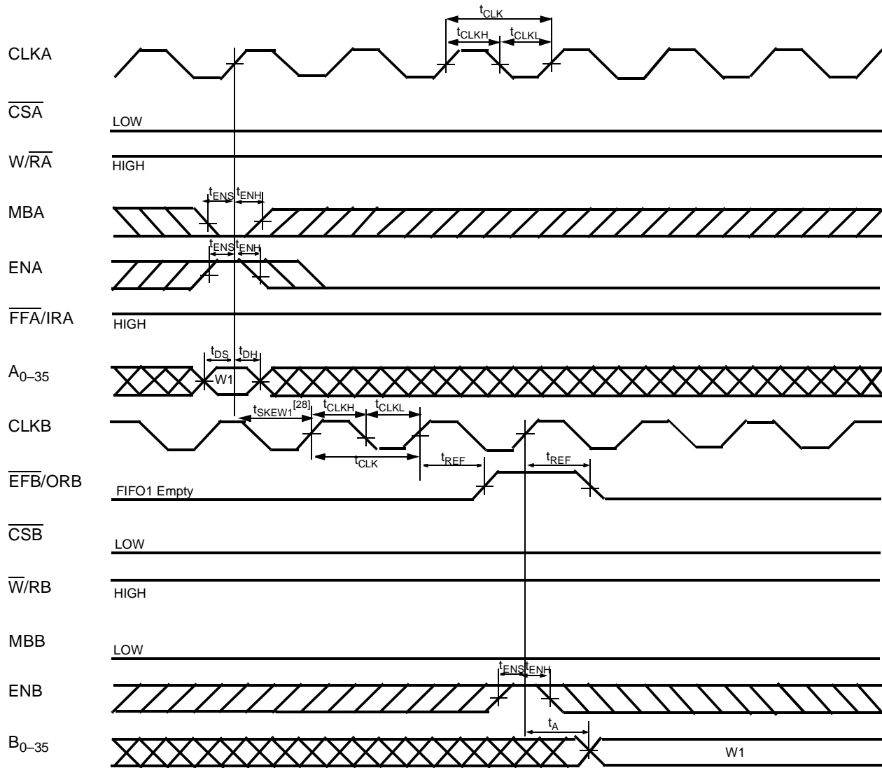
EFB Flag Timing and First Data Read Fall Through when FIFO1 is Empty (CY standard Mode) [26]
