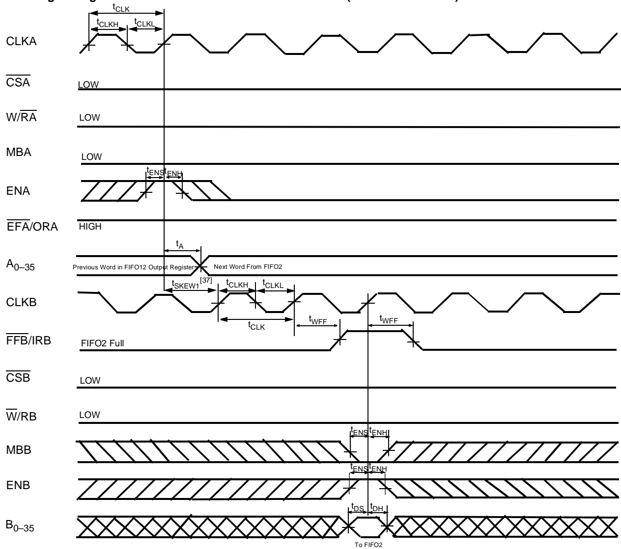
FFB Flag Timing and First Available Write when FIFO2 is Full (CY Standard Mode) [36]
