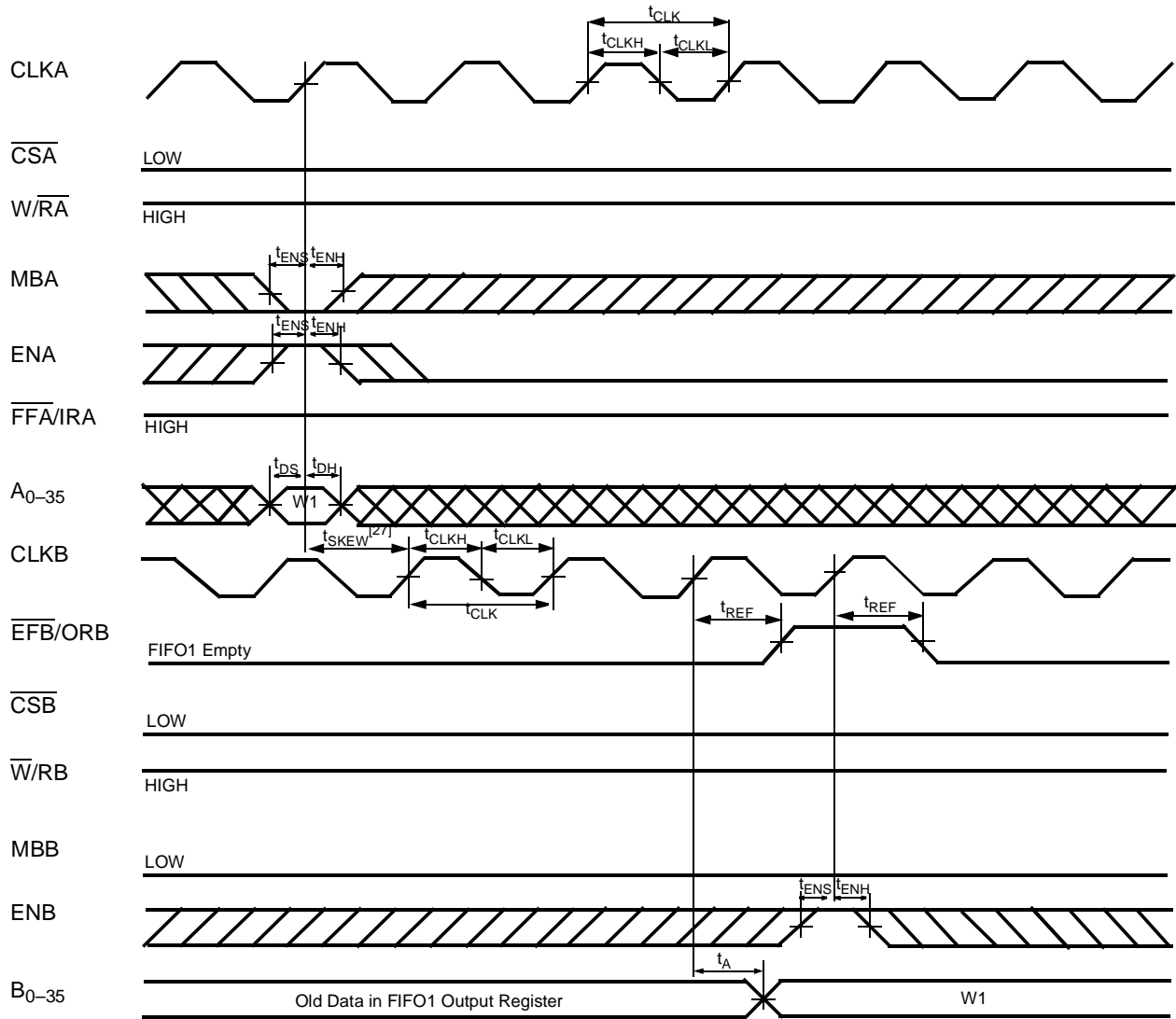
ORB Flag Timing and First Data Word Fall Through when FIFO1 is Empty (FWFT Mode) [22, 26]
