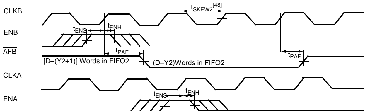
Timing for \overline{\text{AFB}} when FIFO2 is Almost Full (CY Standard and FWFT Modes) [41, 44, 45, 47]
