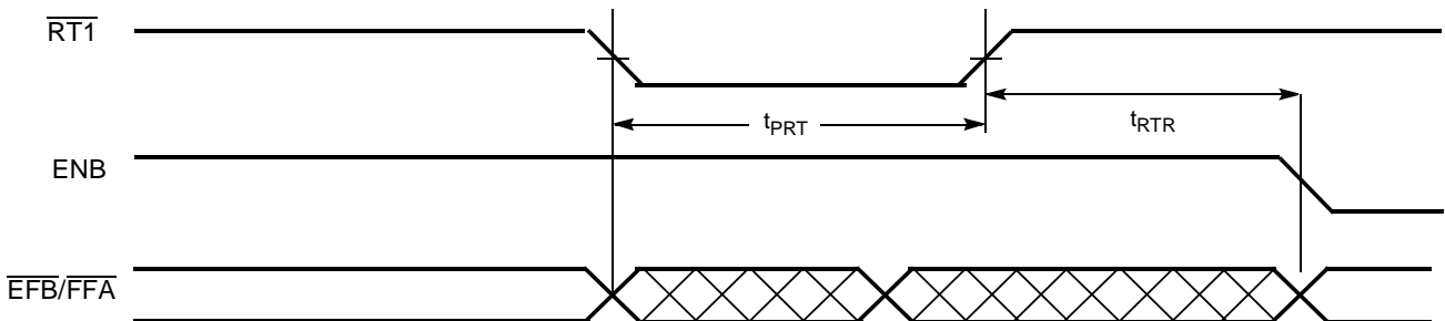
FIFO1 Retransmit Timing [50, 51, 52, 53]
