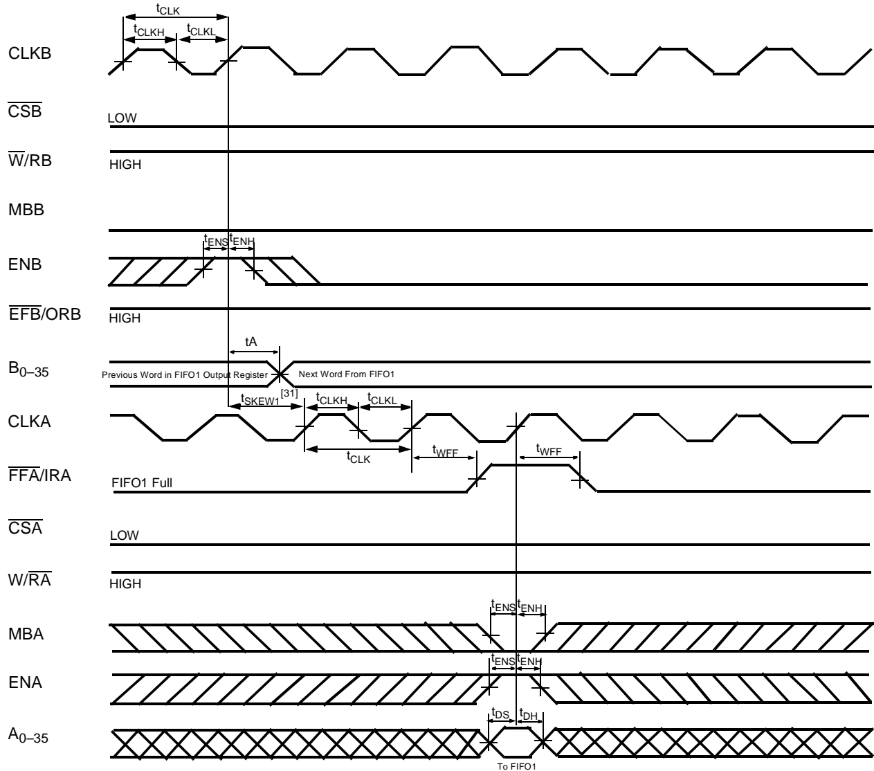
IRA Flag Timing and First Available Write when FIFO1 is Full (FWFT Mode) [28]
