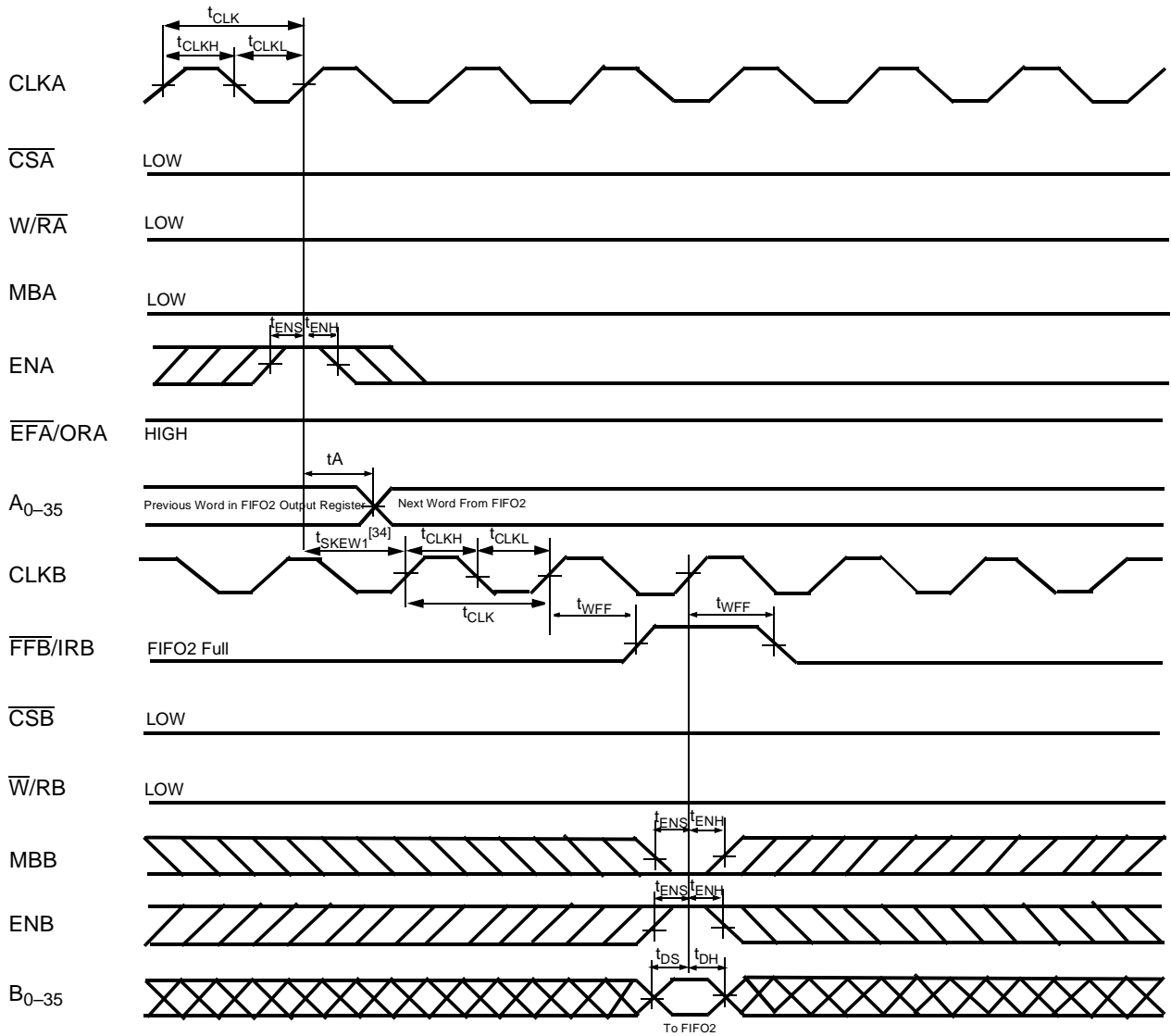
IRB Flag Timing and First Available Write when FIFO2 is Full (FWFT Mode) [33]
