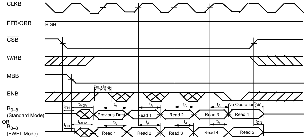
Port B Word Read Cycle Timing for FIFO1 (CY Standard and FWFT Modes) [22]
