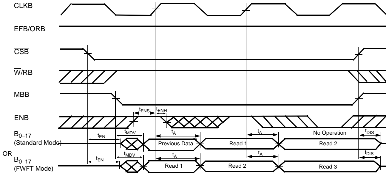
Port B Byte Read Cycle Timing for FIFO1 (CY Standard and FWFT Modes) [23]
