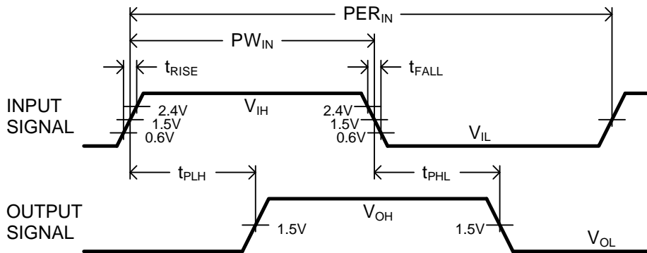
Figure 4: Timing Diagram
