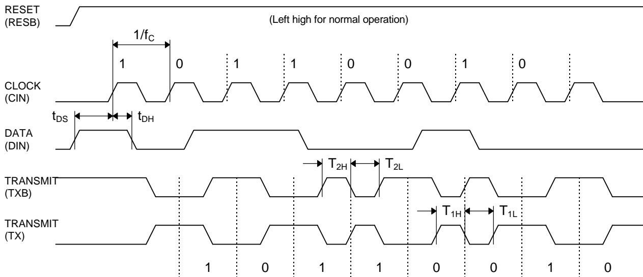
Figure 1: Timing Diagram (Encoder)
