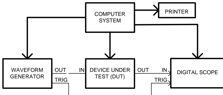
Figure 3: Test Setup
