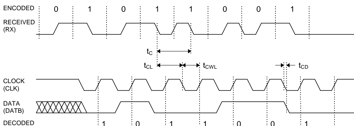
Figure 2: Timing Diagram (Decoder)
