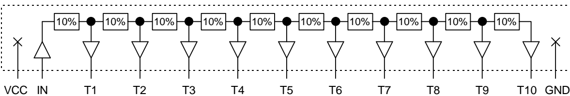
Functional diagram for dash numbers >= 50
