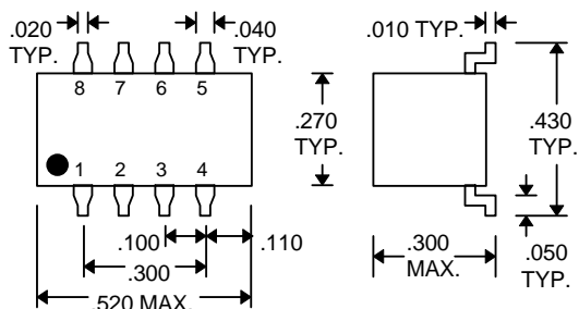
DDU8F-xxA1 (Commercial Gull-Wing)
