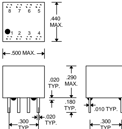
DDU8F-xxM (Military DIP)
