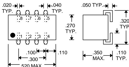
DDU8F-xxB1 (Commercial J-Lead)
