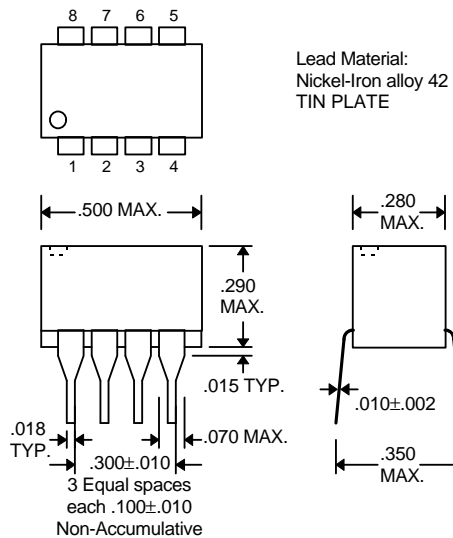
DDU8F-xx (Commercial DIP)
