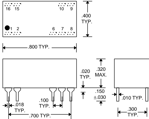
PDU108H-xx (Commercial DIP) PDU108H-xxM (Military DIP)
