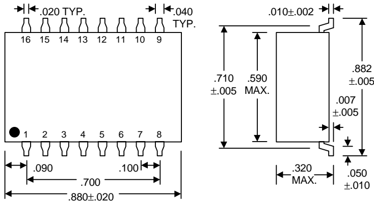
PDU108H-xxC3 (Commercial SMD) PDU108H-xxMC3 (Military SMD)
