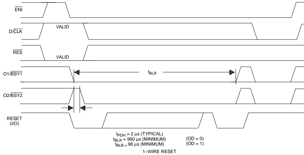
TIMING DIAGRAM: HOST INTERFACE Figure 6
