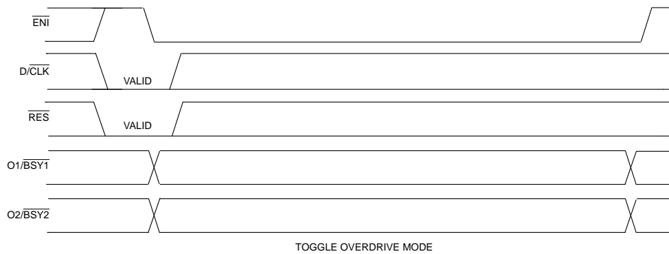
TIMING DIAGRAM: HOST INTERFACE Figure 7
