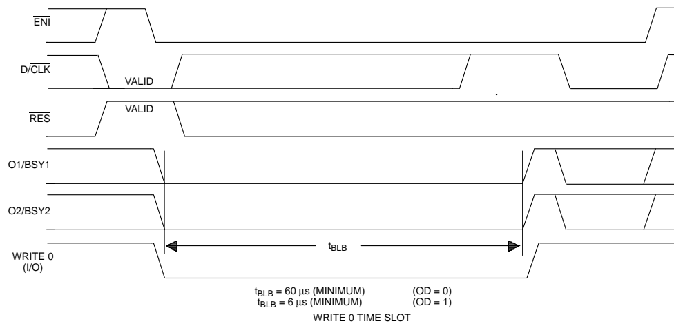
TIMING DIAGRAM: HOST INTERFACE Figure 5
