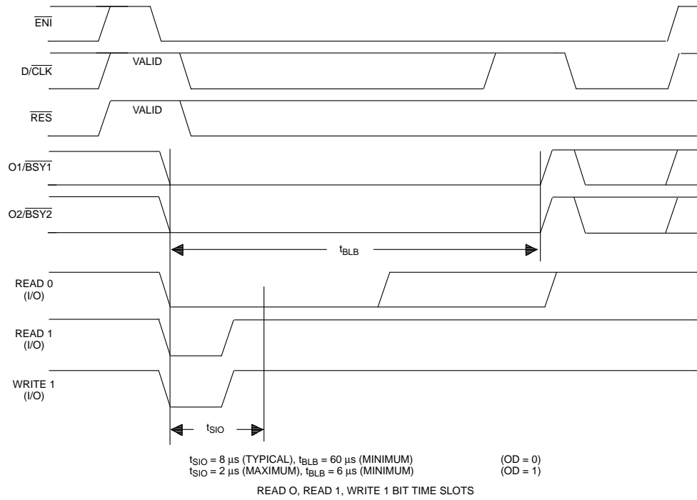
TIMING DIAGRAM: HOST INTERFACE Figure 4
