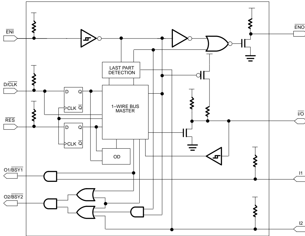
DS1481 FUNCTIONAL BLOCK DIAGRAM Figure 1
