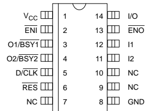
14-PIN SOIC (150 MIL)
