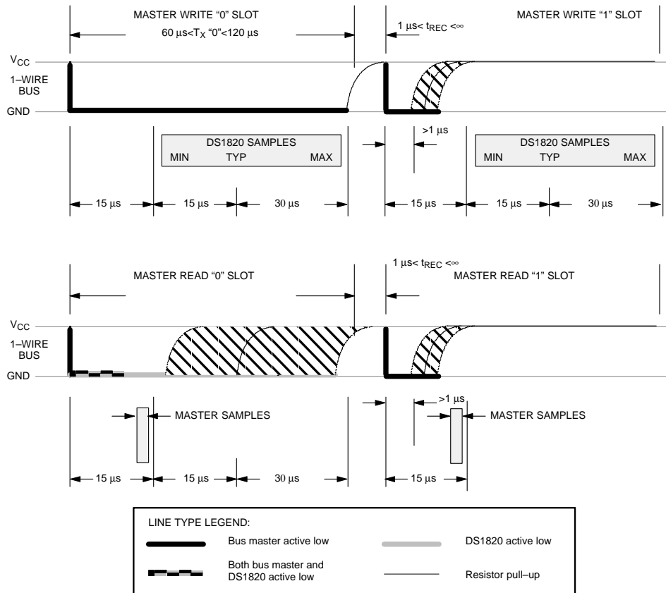
READ/WRITE TIMING DIAGRAM Figure 12
