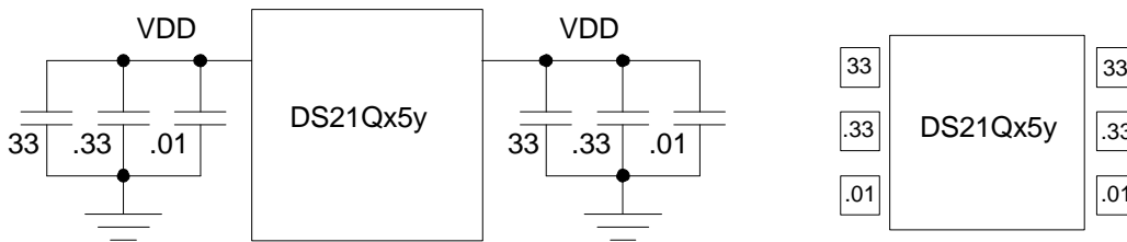
De-coupling scheme using standard tantalum caps. Figure 3
