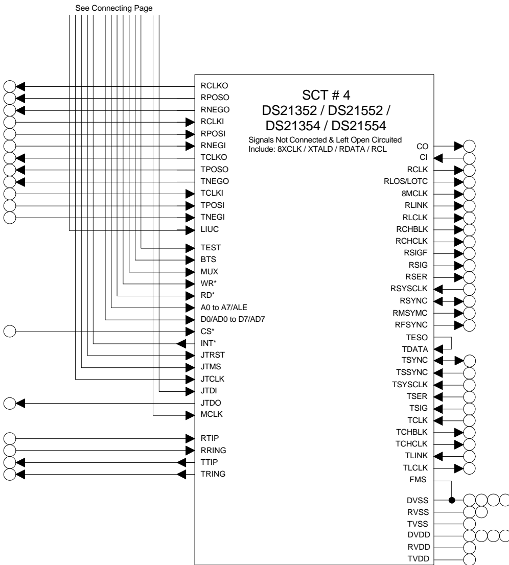
DS21Q352 / DS21Q552 / DS21Q354 / DS21Q554 Schematic Figure 1 (continued)
