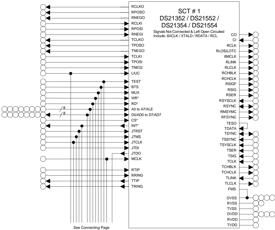
DS21Q352 / DS21Q552 / DS21Q354 / DS21Q554 Schematic Figure 1
