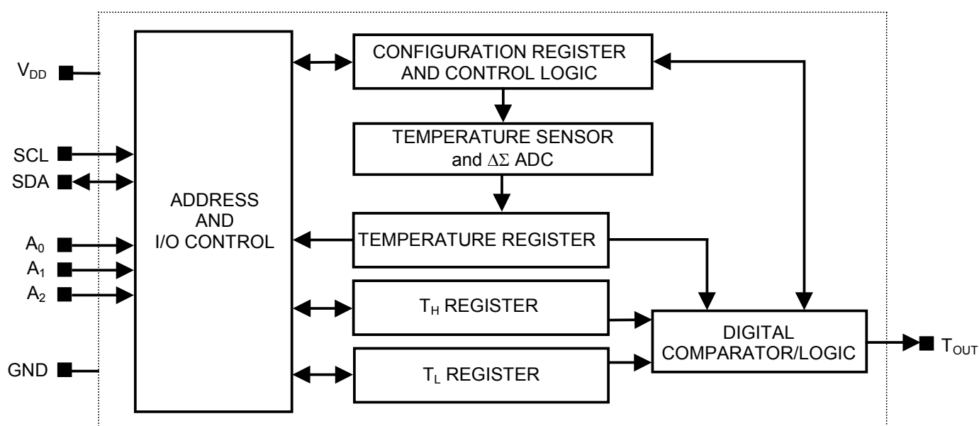
Figure 1. FUNCTIONAL DIAGRAM
