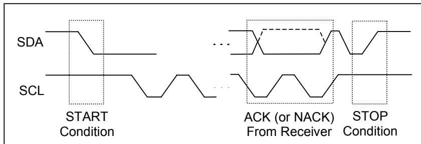
Figure 8. START, STOP, AND ACK SIGNALS
