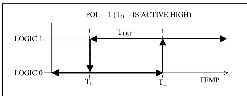
Figure 5. THERMOSTAT OUTPUT OPERATION
