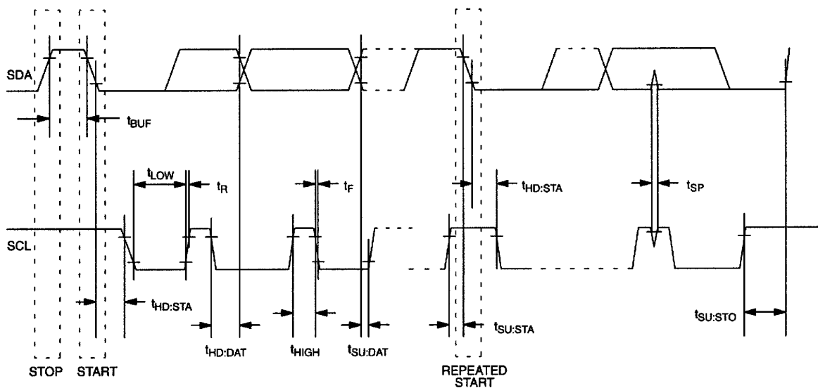
Figure 3. TIMING DIAGRAM
